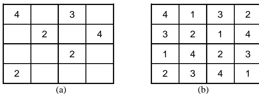
Figure 1. Sample 4 \times 4 Sudoku puzzle and solution
